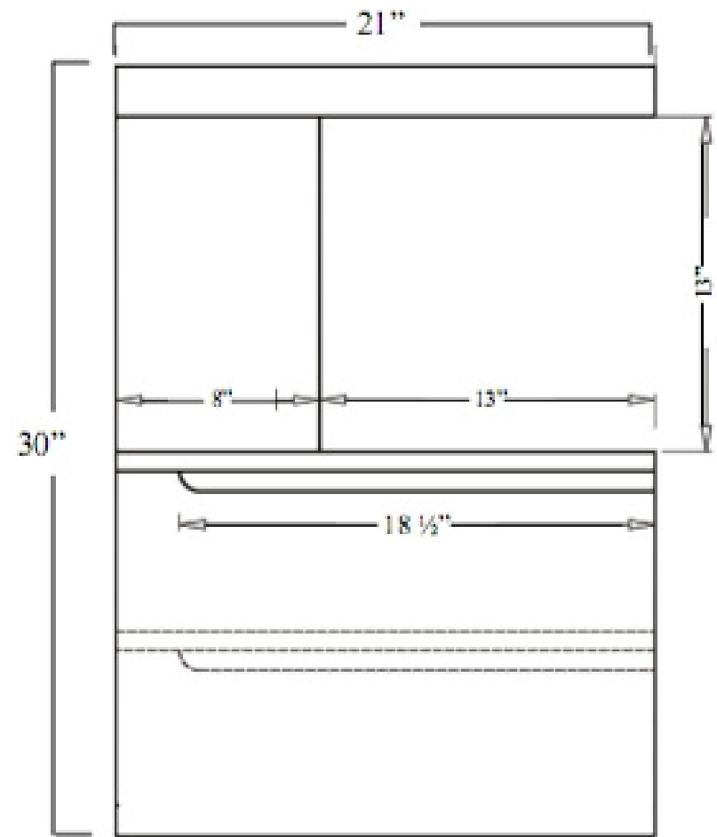
SideView
